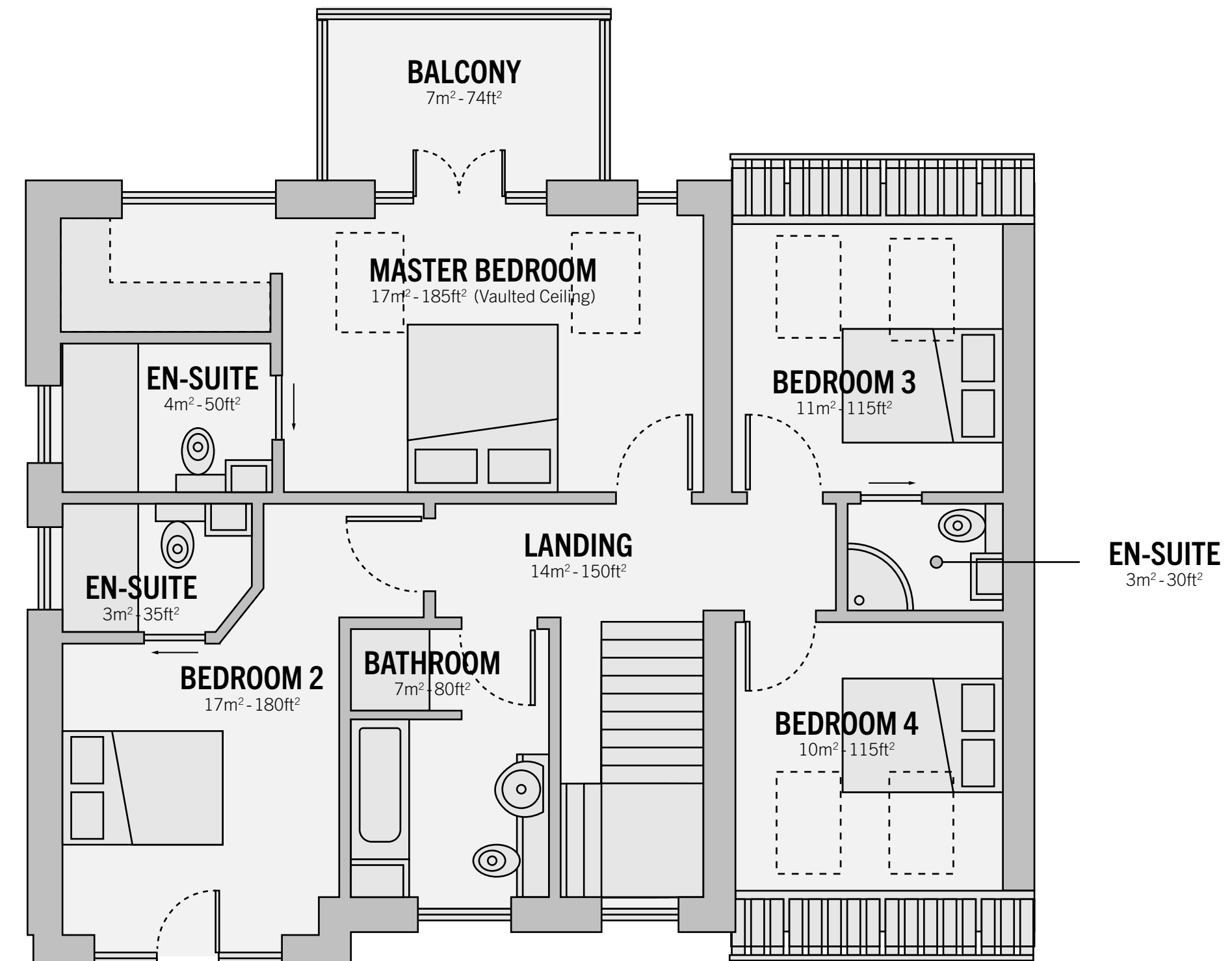
First Floor
